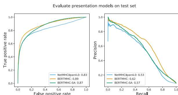
Fig. 6. Comparing BERTMHC, BERTMHC-SA and NetMHCIIpan4.0 on independent mass spectrometry data from IEDB. (left) ROC curve for BERTMHC (yellow), BERTMHC-SA (green) and NetMHCIIpan4.0 (blue). (right) Precision-recall curve for BERTMHC (yellow), BERTMHC-SA (green) and NetMHCIIpan4.0 (blue). The number in the legend gives the area under the curve for that method
